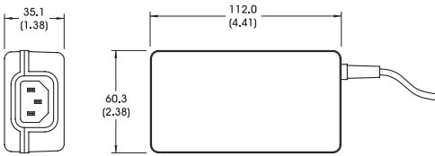
DIMENSION ARE IN MILLIMETERS (INCHES)
